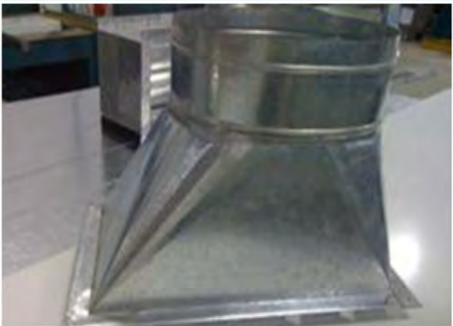
Bottom Plate Square to Round
